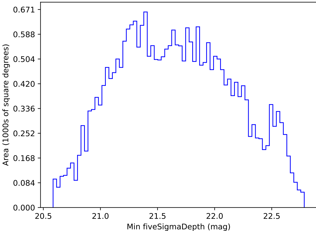
baseline_v3.2_10yrs All sky i band: Min fiveSigmaDepth
