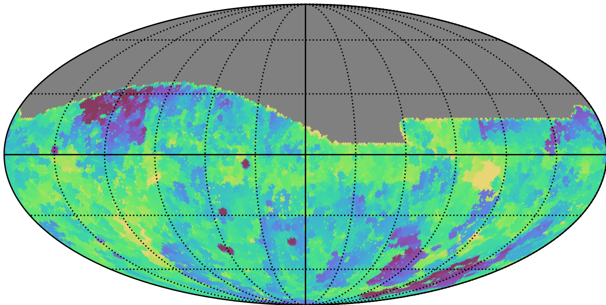
baseline_v3.2_10yrs All sky g band: Min fiveSigmaDepth
