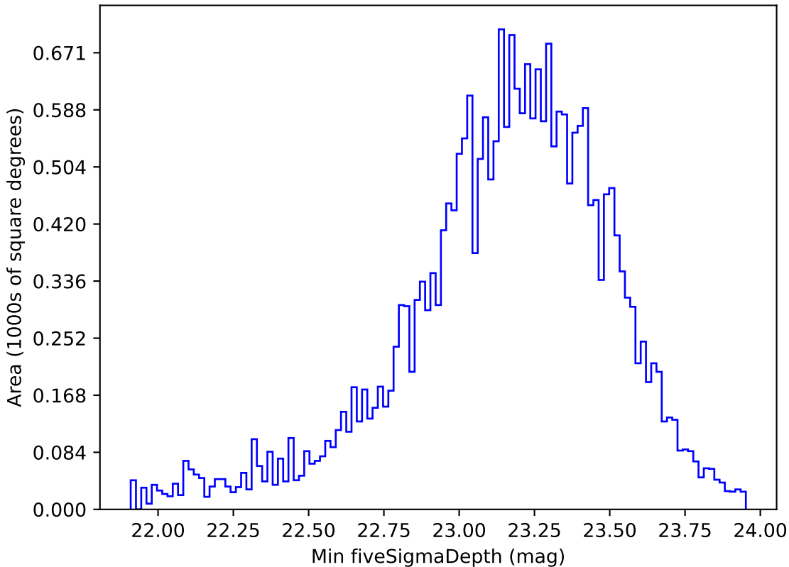
baseline_v3.2_10yrs All sky g band: Min fiveSigmaDepth
