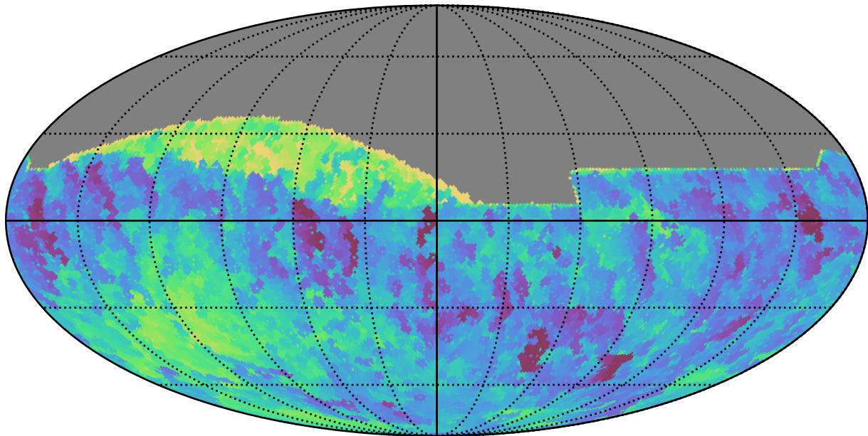
baseline_v3.2_10yrs All sky all bands: Min fiveSigmaDepth
