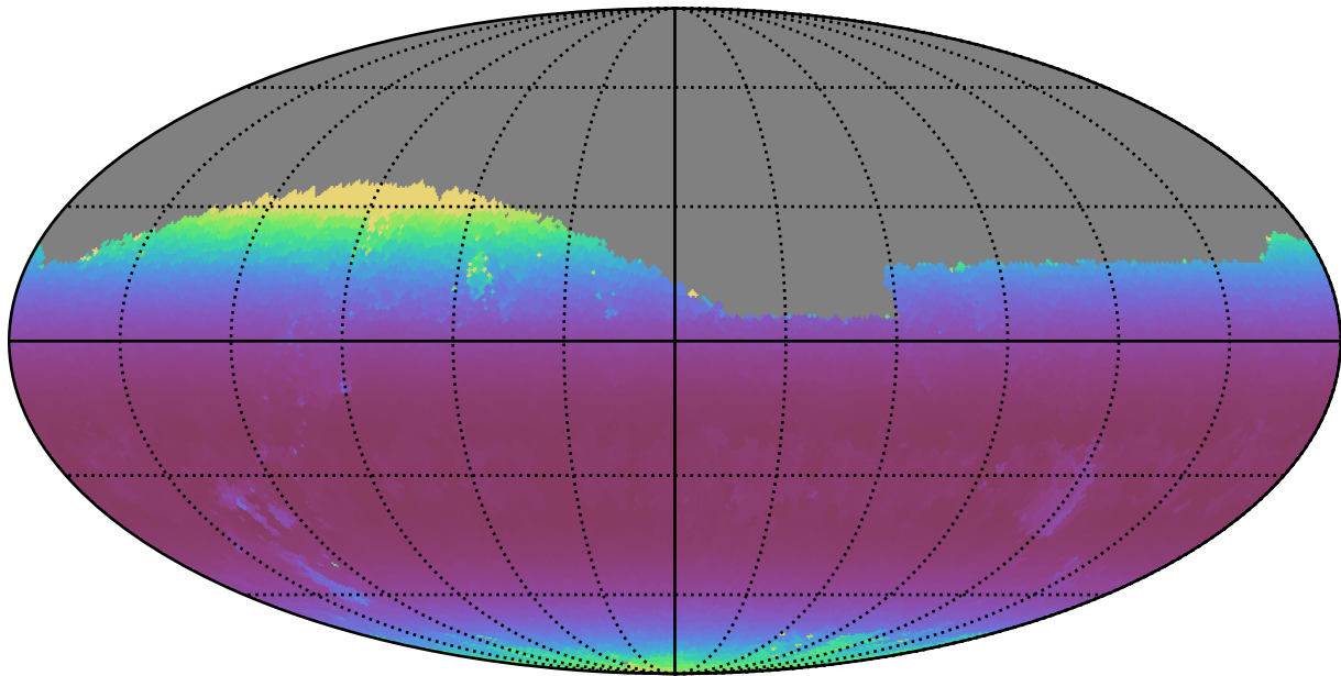
baseline_v3.2_10yrs Yr 1 z band: Min airmass
