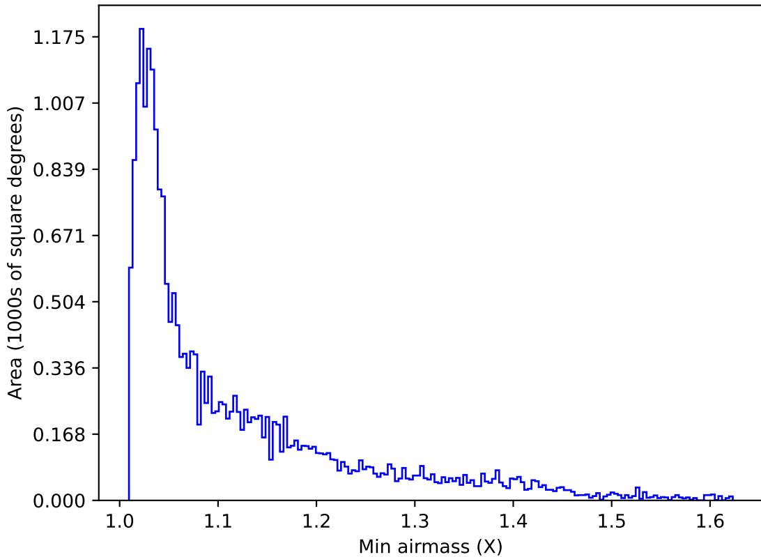
baseline_v3.2_10yrs Yr 1 y band: Min airmass
