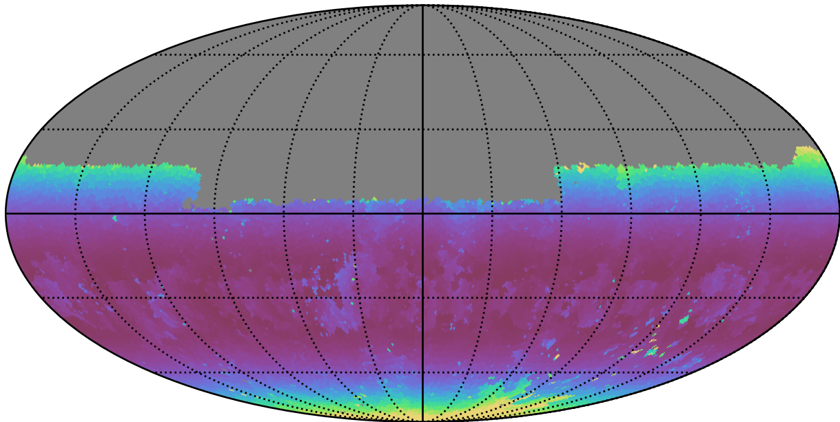
baseline_v3.2_10yrs Yr 1 u band: Min airmass
