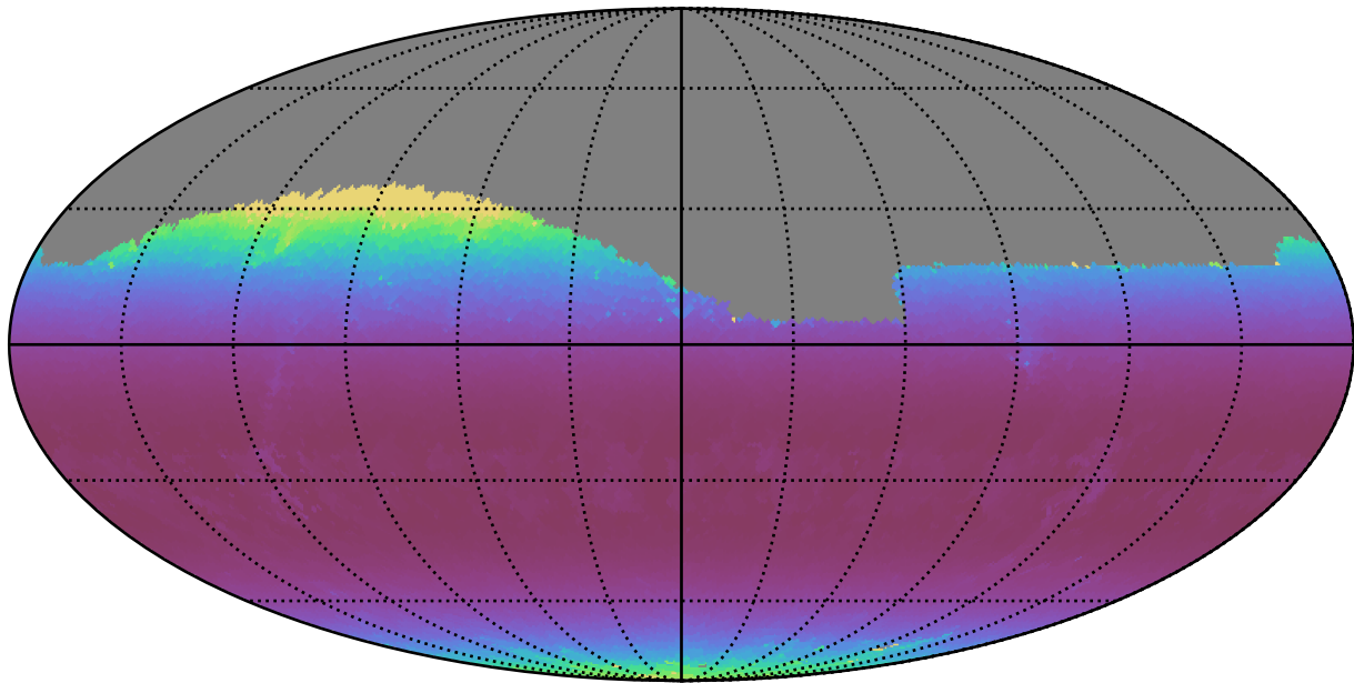
baseline_v3.2_10yrs Yr 1 r band: Min airmass
