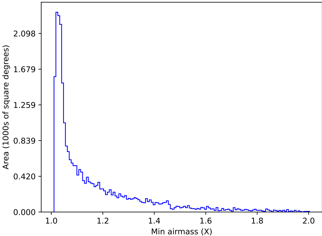
baseline_v3.2_10yrs Yr 1 r band: Min airmass
