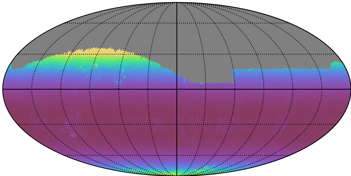
baseline_v3.2_10yrs Yr 1 i band: Min airmass
