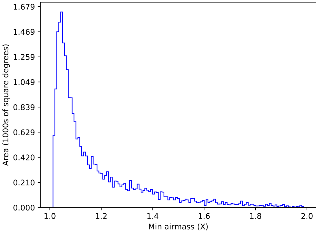
baseline_v3.2_10yrs Yr 1 g band: Min airmass
