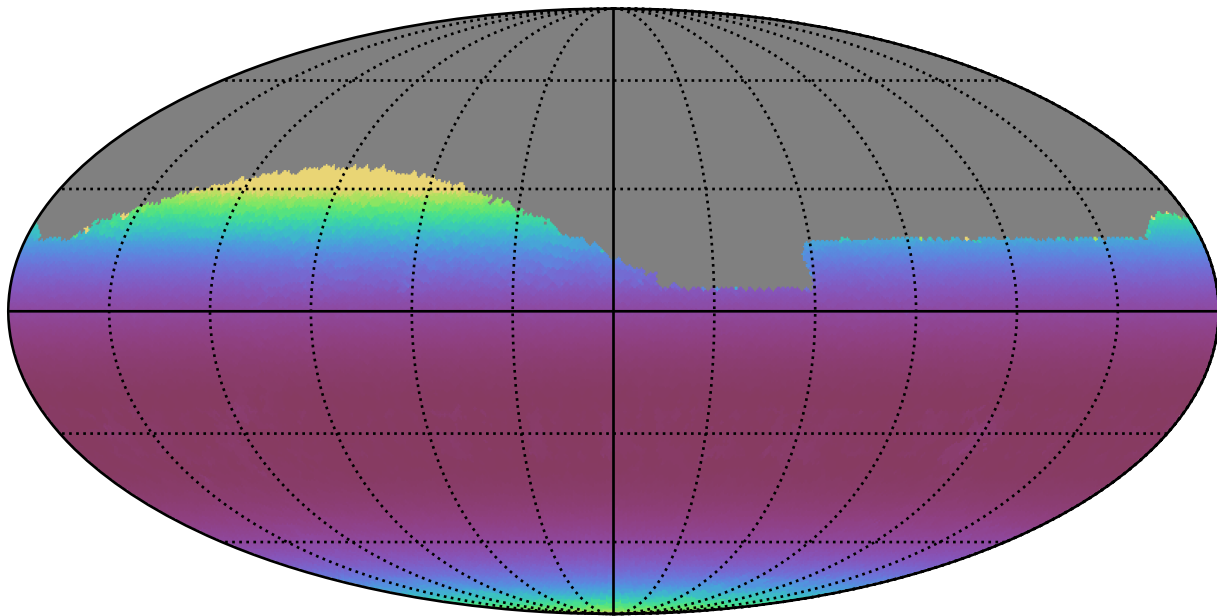
baseline_v3.2_10yrs Yr 1 all bands: Min airmass
