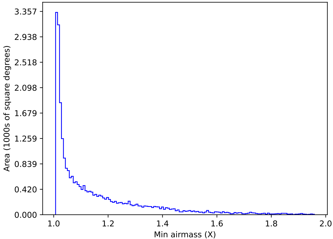
baseline_v3.2_10yrs Yr 1 all bands: Min airmass
