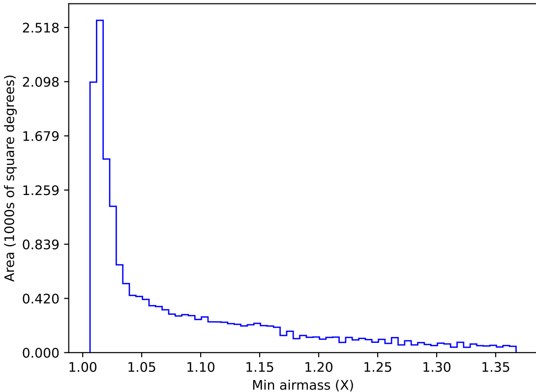
baseline_v3.2_10yrs WFD z band: Min airmass
