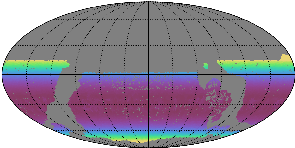
baseline_v3.2_10yrs WFD y band: Min airmass
