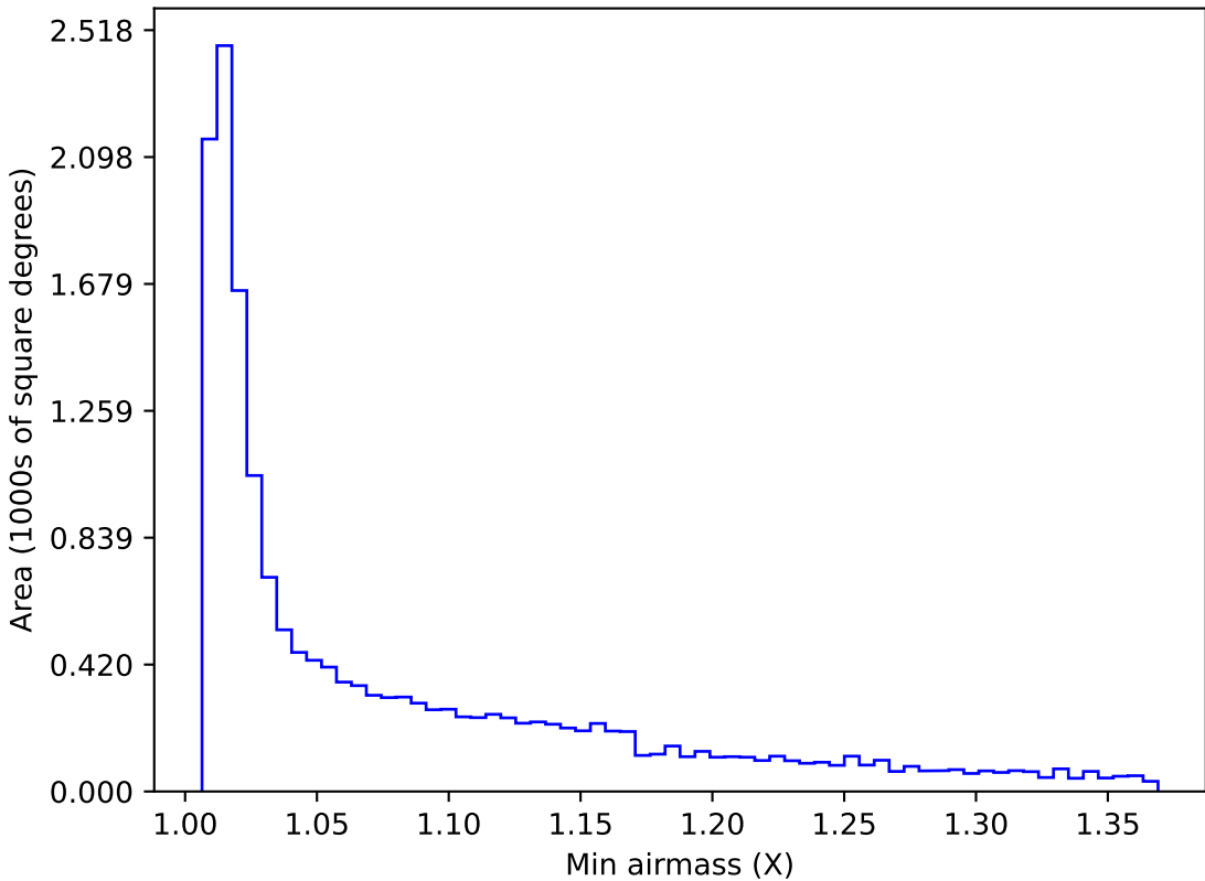
baseline_v3.2_10yrs WFD y band: Min airmass
