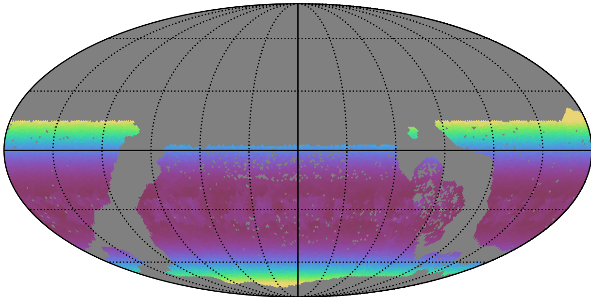
baseline_v3.2_10yrs WFD u band: Min airmass
