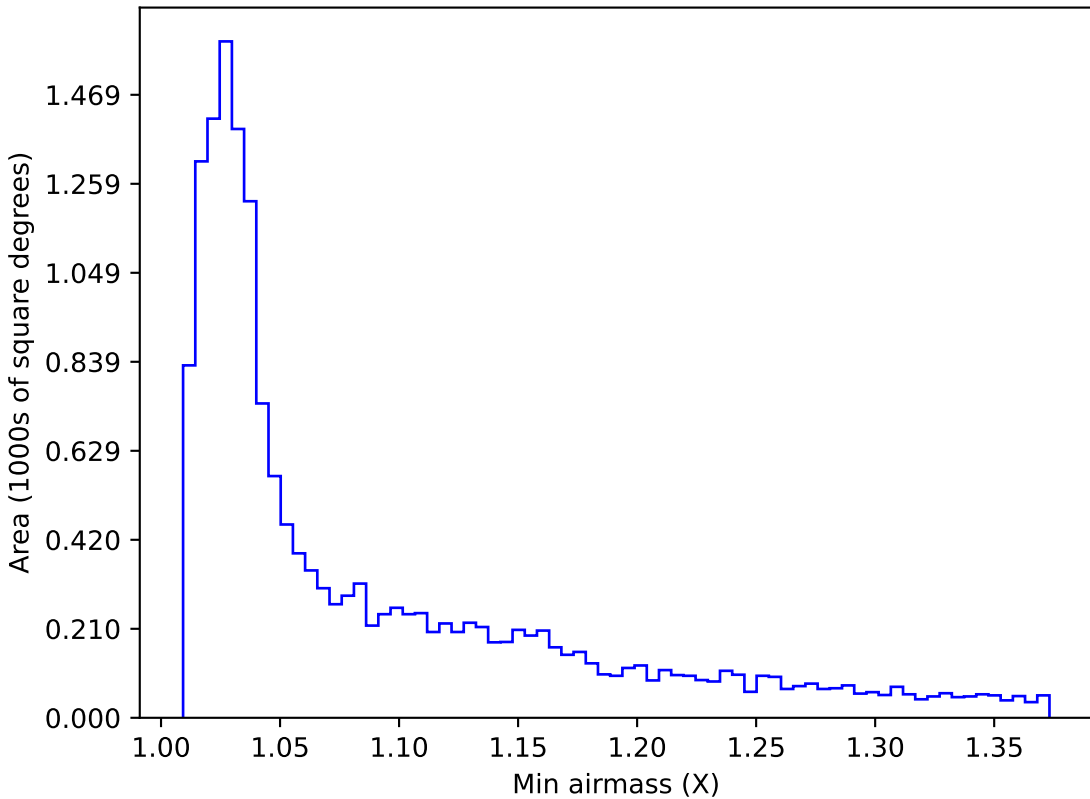
baseline_v3.2_10yrs WFD u band: Min airmass
