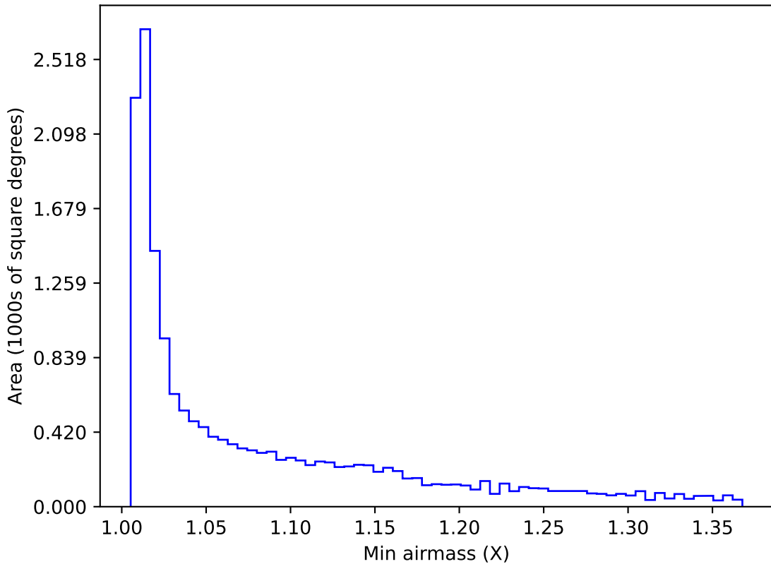
baseline_v3.2_10yrs WFD r band: Min airmass
