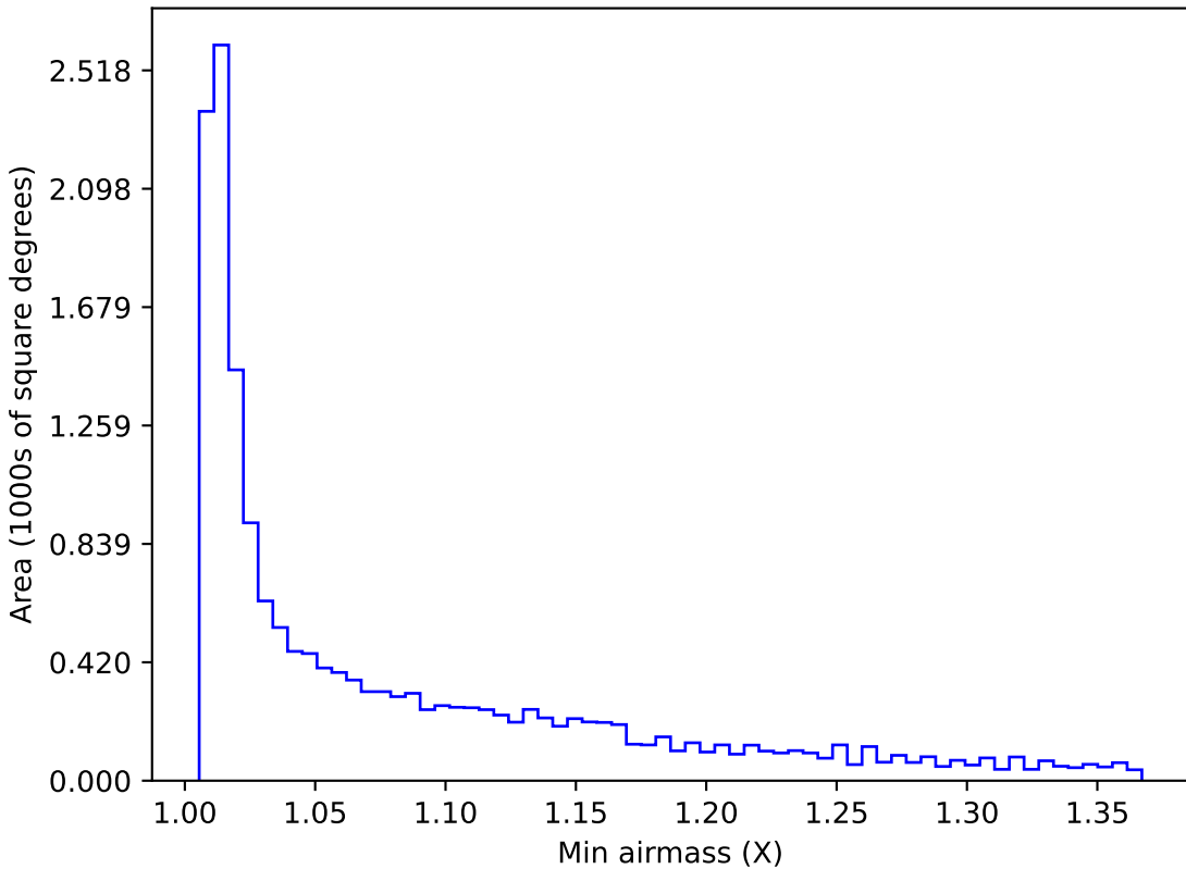
baseline_v3.2_10yrs WFD i band: Min airmass
