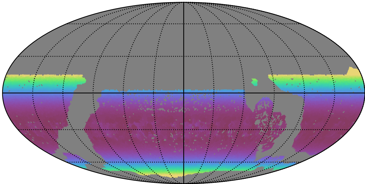
baseline_v3.2_10yrs WFD g band: Min airmass
