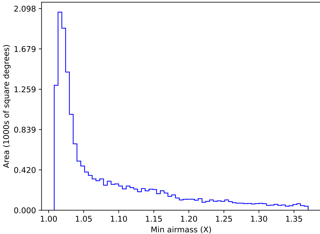
baseline_v3.2_10yrs WFD g band: Min airmass
