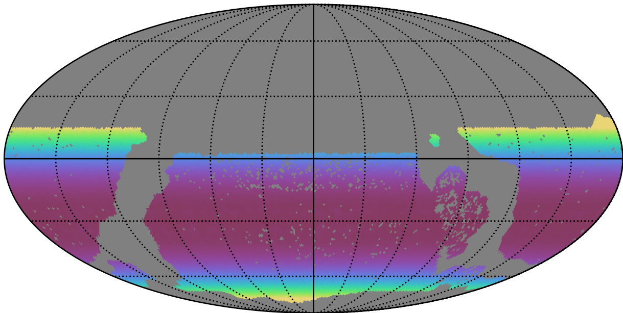
baseline_v3.2_10yrs WFD all bands: Min airmass
