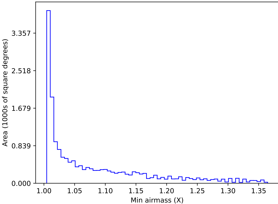
baseline_v3.2_10yrs WFD all bands: Min airmass
