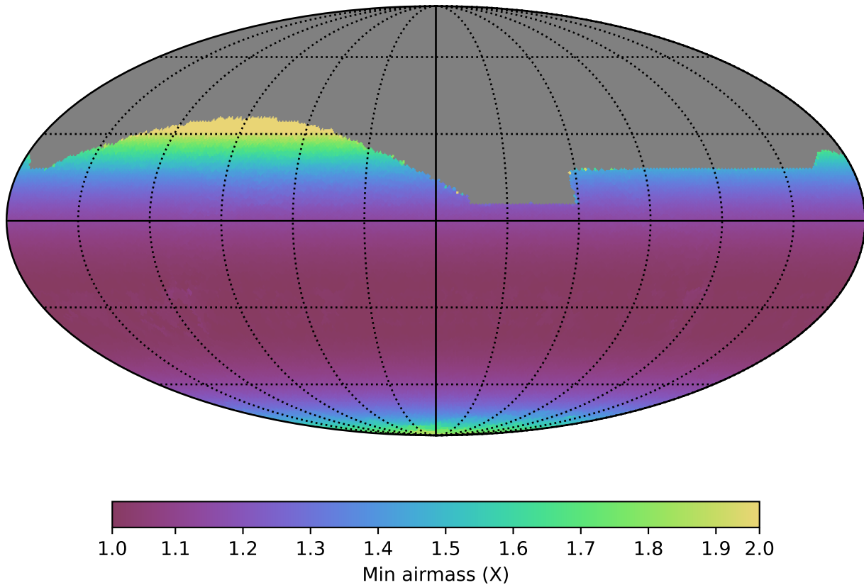
baseline_v3.2_10yrs All sky z band: Min airmass
