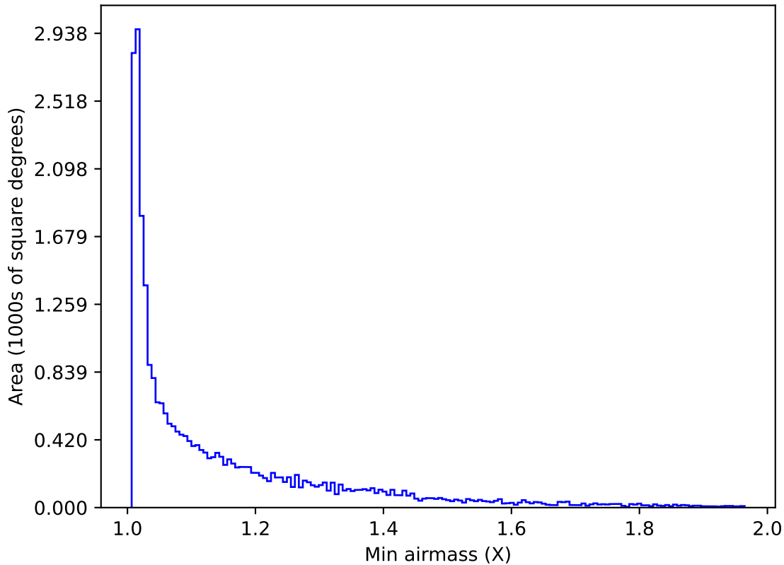
baseline_v3.2_10yrs All sky z band: Min airmass
