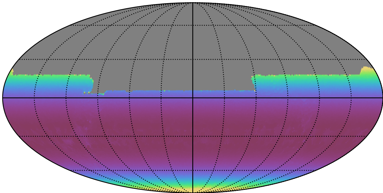
baseline_v3.2_10yrs All sky y band: Min airmass
