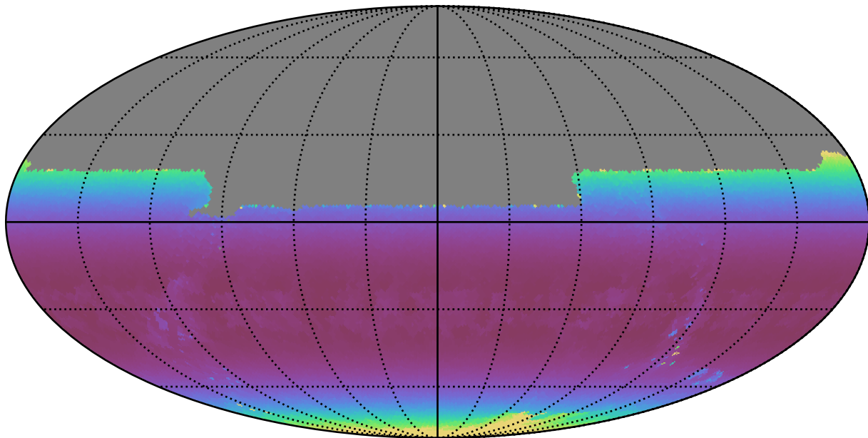
baseline_v3.2_10yrs All sky u band: Min airmass
