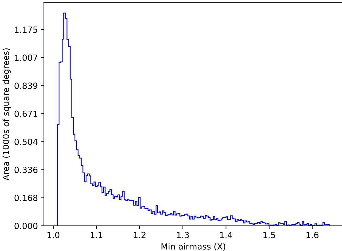
baseline_v3.2_10yrs All sky u band: Min airmass
