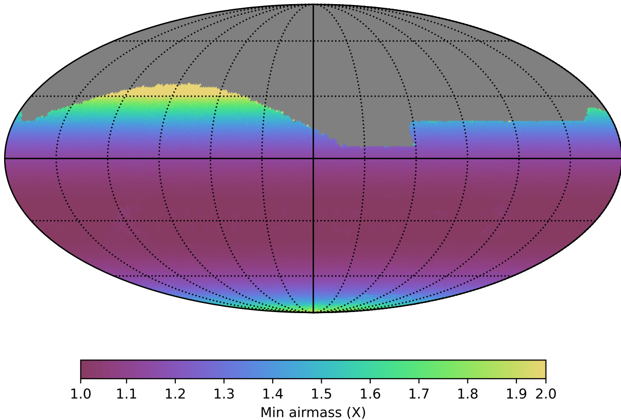
baseline_v3.2_10yrs All sky r band: Min airmass
