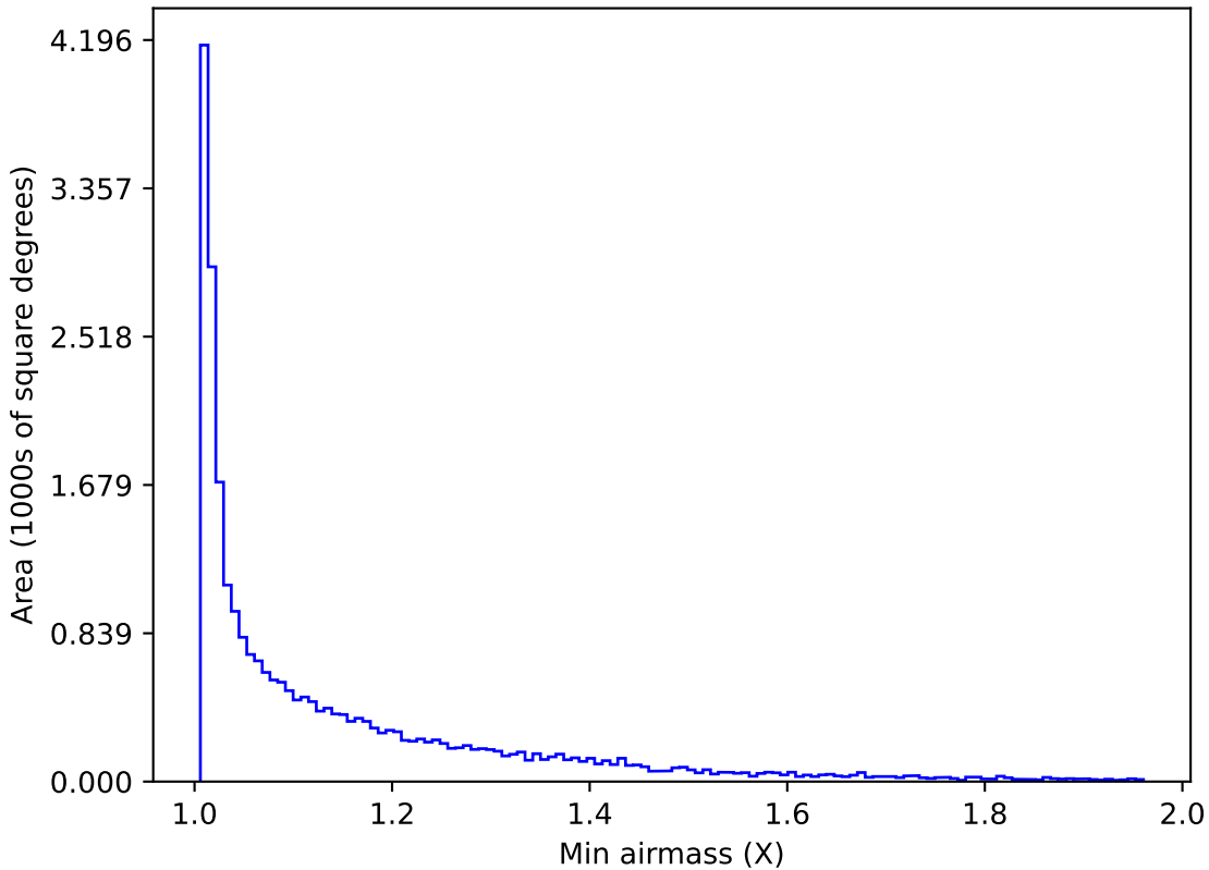
baseline_v3.2_10yrs All sky r band: Min airmass
