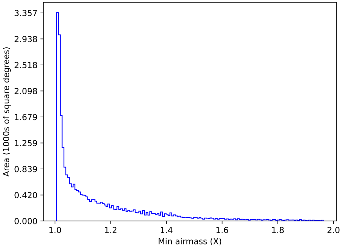
baseline_v3.2_10yrs All sky i band: Min airmass
