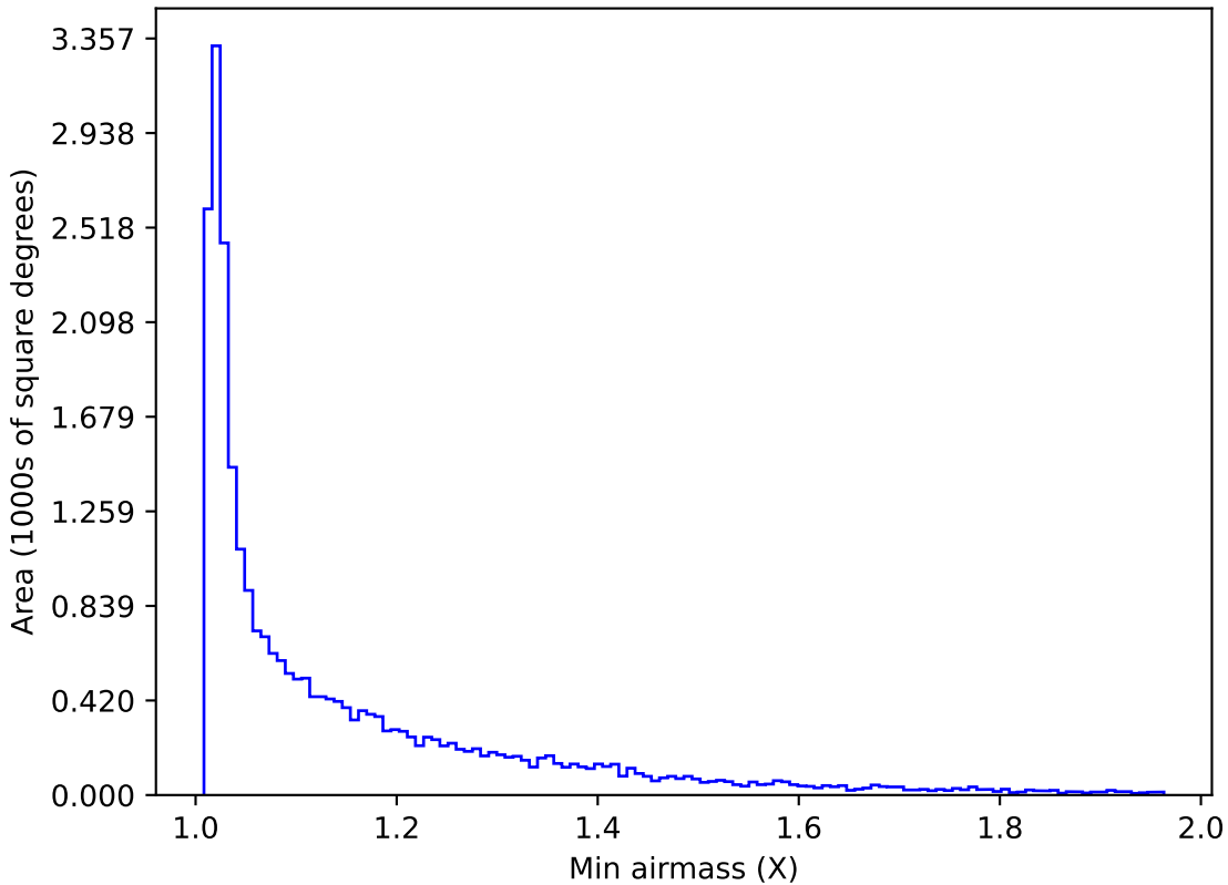
baseline_v3.2_10yrs All sky g band: Min airmass
