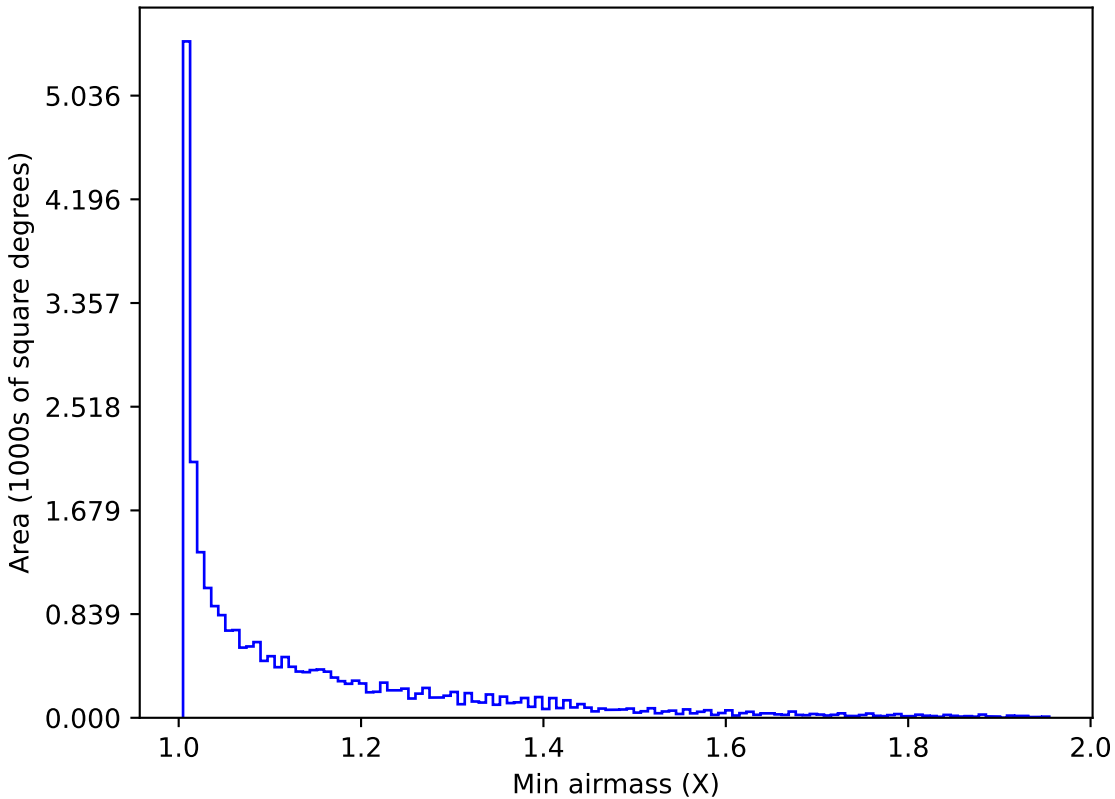
baseline_v3.2_10yrs All sky all bands: Min airmass
