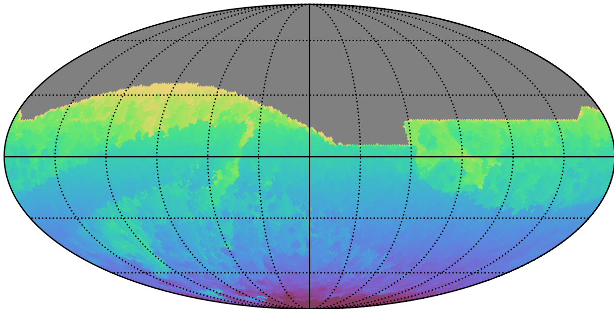
baseline_v3.2_10yrs All sky all bands: Min HA
