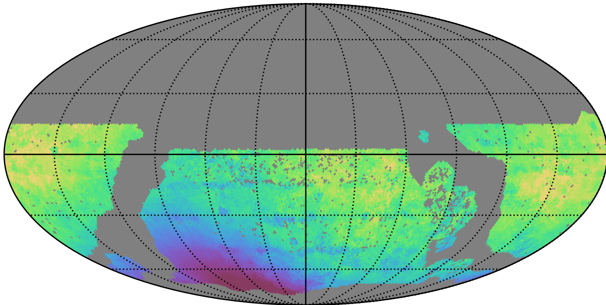
baseline_v3.2_10yrs WFD z band: Median solarElong
