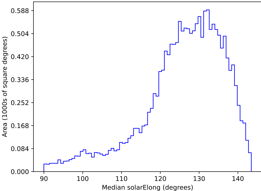
baseline_v3.2_10yrs WFD z band: Median solarElong
