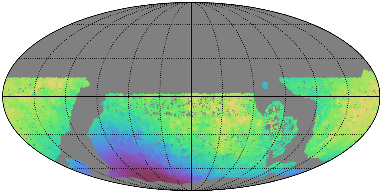
baseline_v3.2_10yrs WFD y band: Median solarElong
