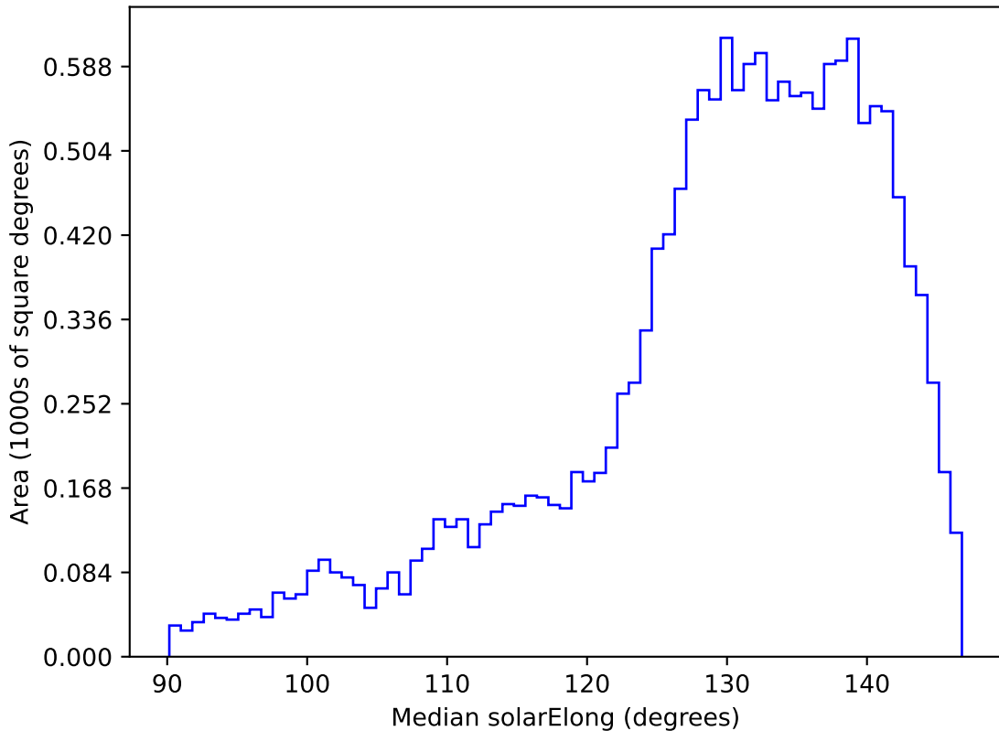
baseline_v3.2_10yrs WFD y band: Median solarElong
