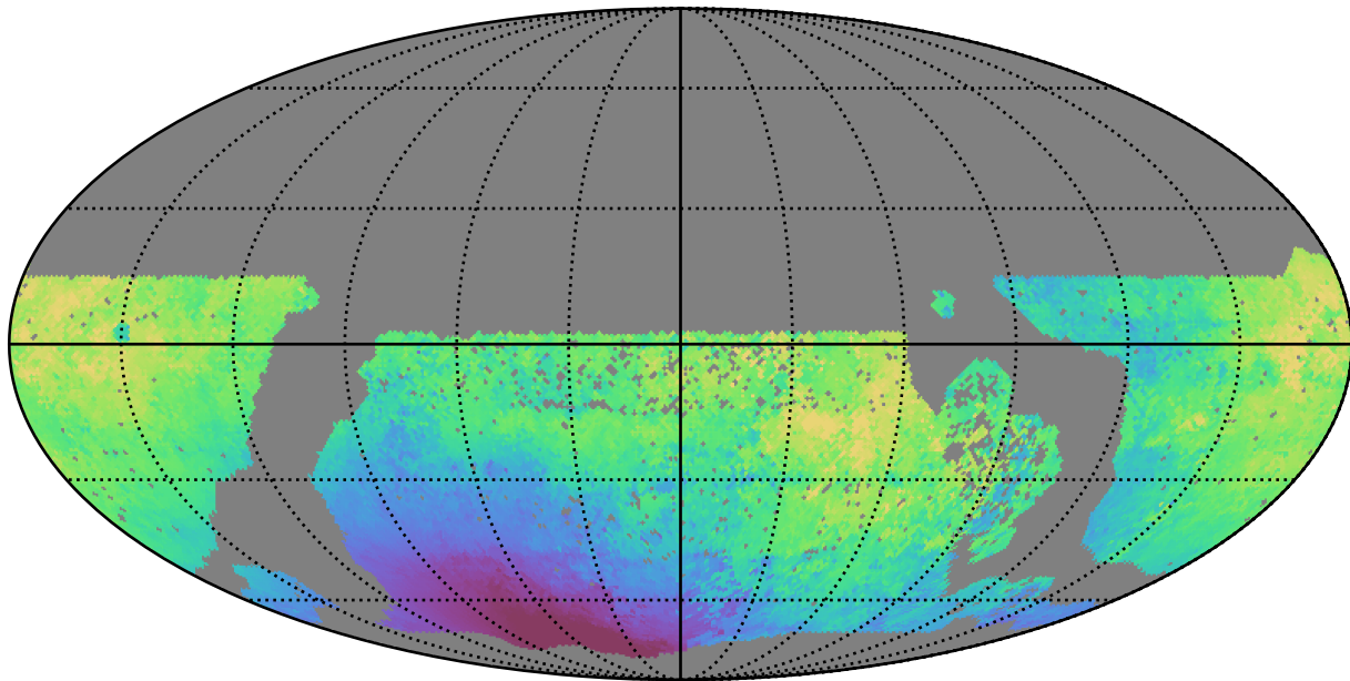
baseline_v3.2_10yrs WFD u band: Median solarElong
