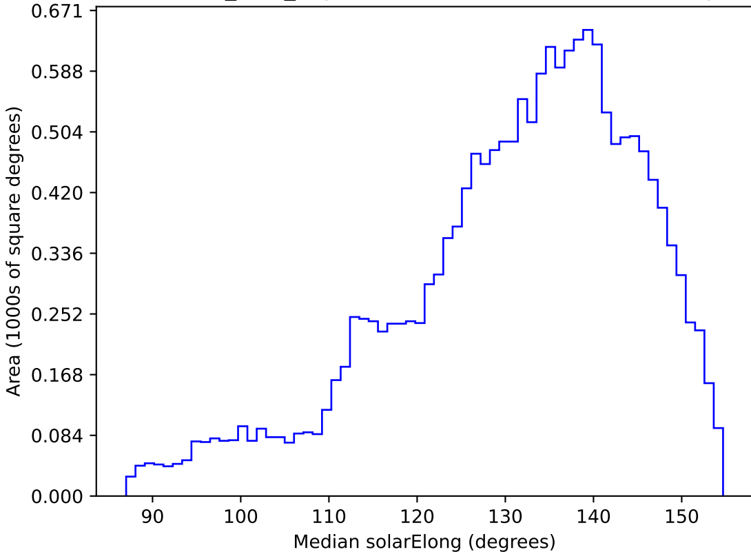
baseline_v3.2_10yrs WFD u band: Median solarElong
