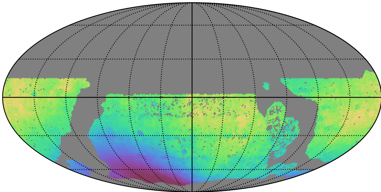
baseline_v3.2_10yrs WFD i band: Median solarElong
