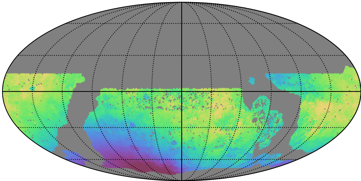
baseline_v3.2_10yrs WFD g band: Median solarElong
