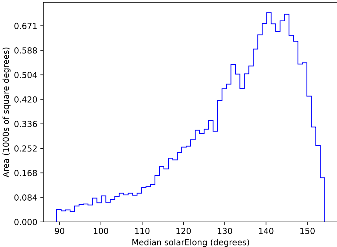
baseline_v3.2_10yrs WFD g band: Median solarElong
