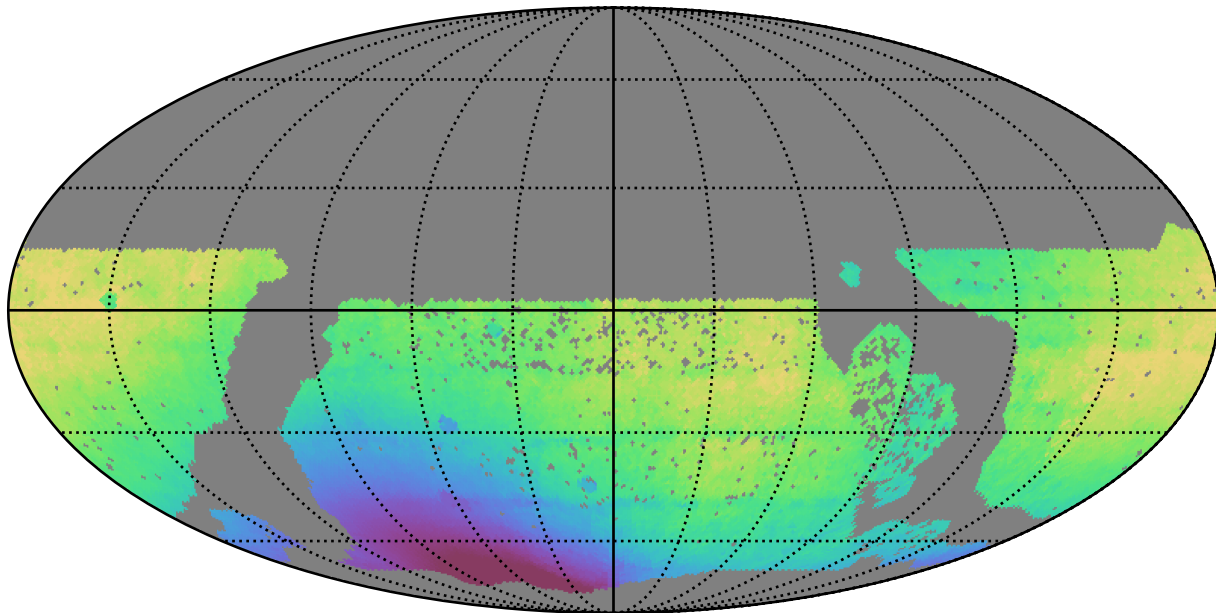
baseline_v3.2_10yrs WFD all bands: Median solarElong
