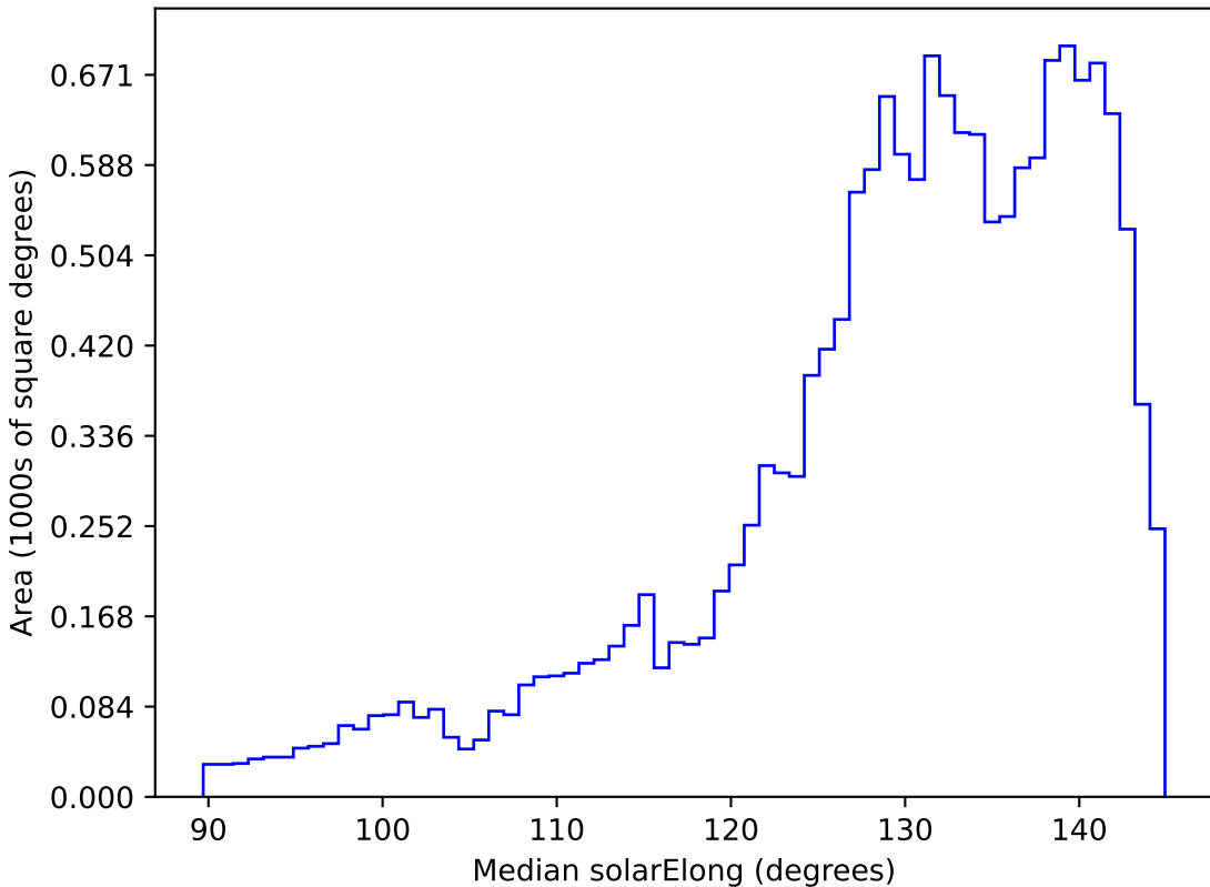
baseline_v3.2_10yrs WFD all bands: Median solarElong
