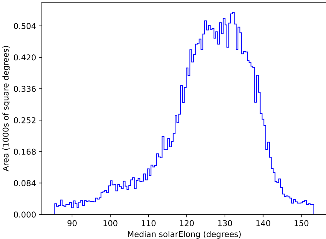
baseline_v3.2_10yrs All sky z band: Median solarElong
