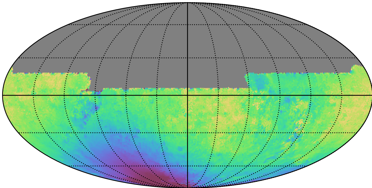
baseline_v3.2_10yrs All sky y band: Median solarElong
