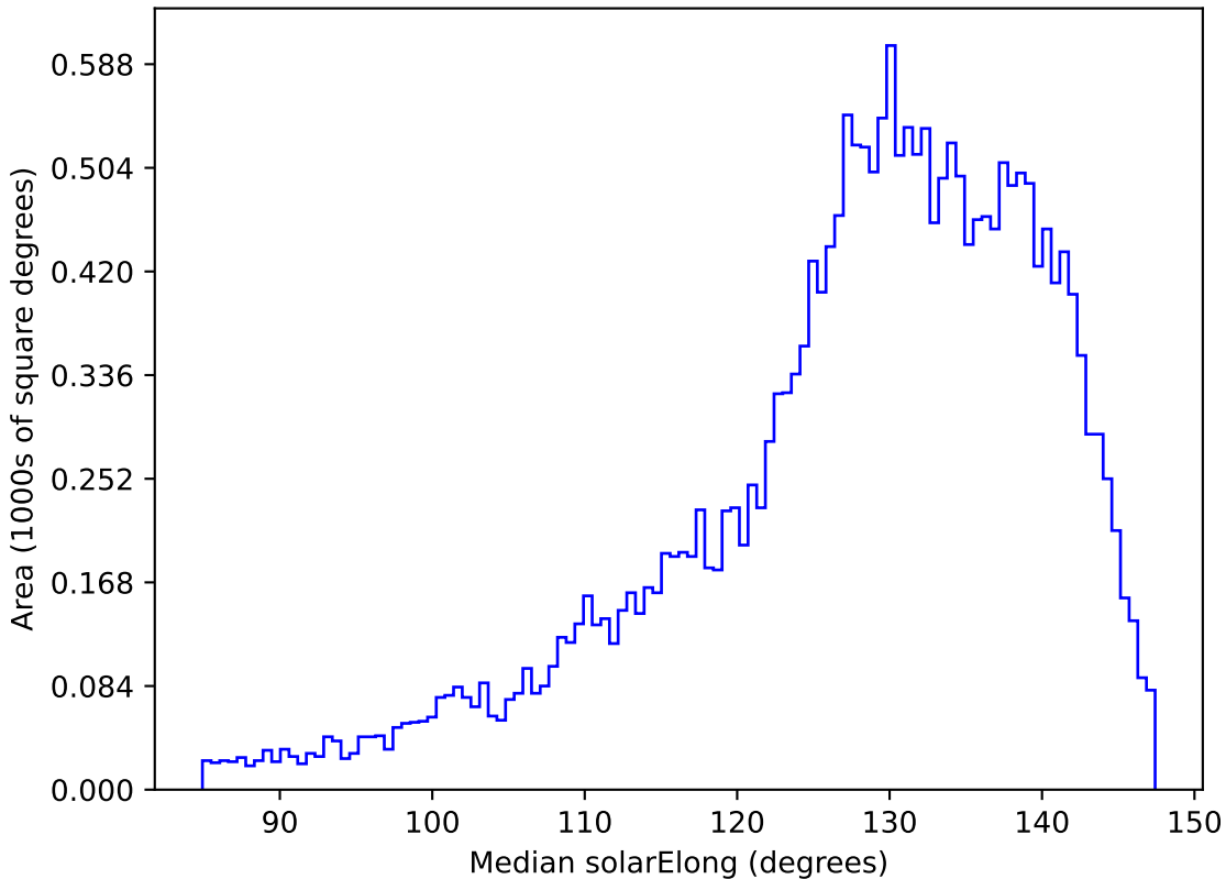
baseline_v3.2_10yrs All sky y band: Median solarElong
