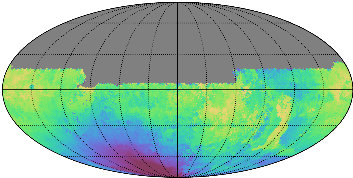
baseline_v3.2_10yrs All sky u band: Median solarElong
